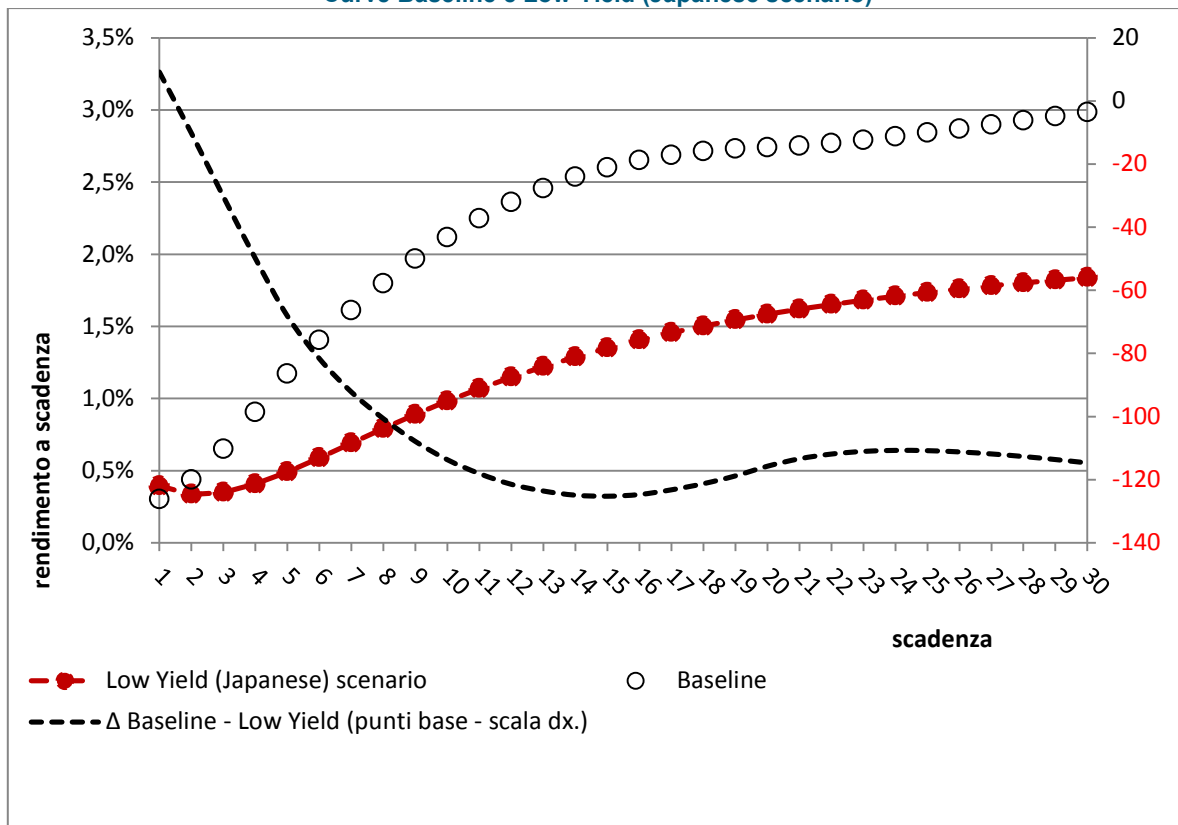
Figura I. 28 - Eiopa Stress-Test 2014 Curve Baseline e Low Yield (Japanese scenario)
